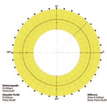
Roundness after Microfinishing
