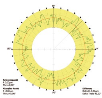
Roundness before Microfinishing
