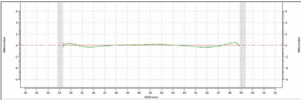
Cross profile: Pt 0.7200 \mu m
