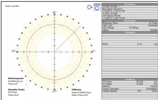
Roundness: 0.16 \mu m, filter 2–200
